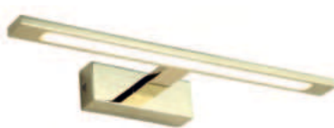
ALTER | Wall lamp W89443-12W-GD LED 12W 1400LM 4000K W50 L415 H135 metal gold body
