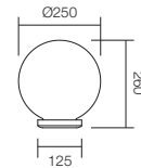
9770 Smoky 9771 Opal E27, 1 x max. 42W
