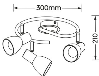
Strahler · Spot incl. 3 x LED E14 3 x 5 W / 3 x 470 Lumen 3.000 Kelvin 871090307 871090308
