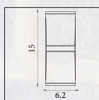
36170BK Montana- LED Outdoor Adjustable Wall Light Black Metal & Polycarbonate
