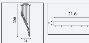
888-8 Sculptured Ice- 8Lt Multi Drop Pendant Chrome Metal & Glass
