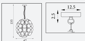
3074-4BG Discus- 4Lt Pendant Black Metal, Black & Gold PC Discs
