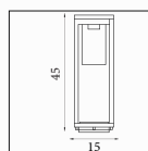
28731-450 Atlanta- Outdoor Post Vandal Proof Black Metal & Polycarbonate
