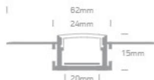
7906TR/AL | 2m Trimless profile + PC opal diffuser | Aluminium | Suitable for 7875 & 7880 LED Strips 37mm
