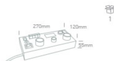
062002 | Display box for LED strips 7820/W, 7820W/W, 7829/C, 7835/W, 7835W/C, 7823/W, 7825/W, 7870/W & 7845/W
