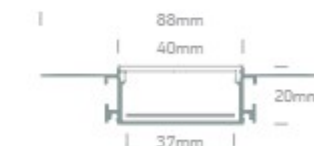
7904ATR/AL | 2m Trimless profile + PC opal diffuser | Aluminium | Suitable for 7820, 7829, 7835, 7845, 7846, 7875 & 7887 LED Strips 20mm
