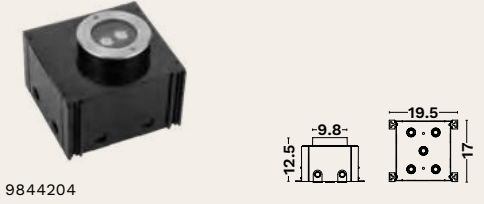
MOUNTING SLEEVE
