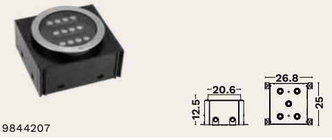
MOUNTING SLEEVE
