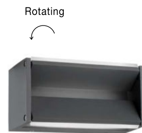
TWIN • 713122 Dark Gray Aluminium Acrylic Diffuser LED 2x5 Watt 476Lm 3000K 220-240 Volt Rotation 0-90° IP54 L: 20 W: 10 H: 10 cm
