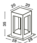
BEV • 9540215 Gray Cement Glass Diffuser LED 5 Watt 200Lm 3000K 120-230V IP65 L: 20 W: 20 H: 35 cm
