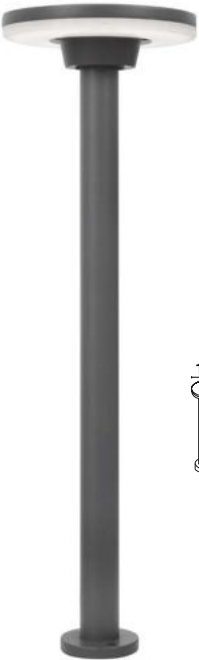
SUITE . 9207167 Dark Gray Aluminium & Acrylic LED 12 Watt 480Lm 3000K 100-240 Volt 50Hz Beam 140° IP54 D: 18 H: 60 cm
