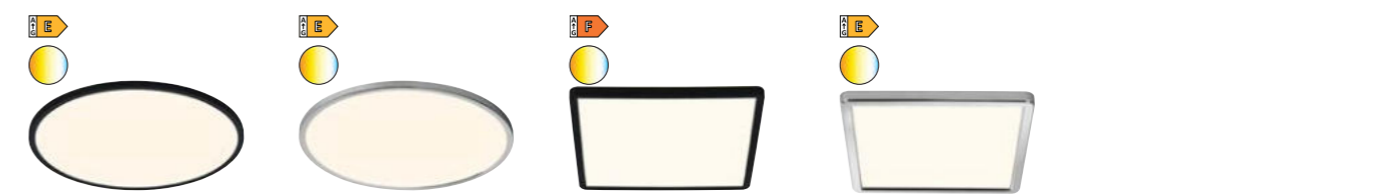
Oja 42 2015116103 Black | Plastic | LED Module 19W 2100lm | 3000/4000K H: 2,3 cm | Ø: 42,4 cm Oja 42 2015116133 Chrome | Plastic | LED Module 19W 2100lm | 3000/4000K H: 2,5 cm | Ø: 43 cm Oja 29 2015066103 Black | Plastic | LED Module 14,5W 1600lm | 3000/4000K H: 2,3 cm | Oja 29 2015066133 Chrome | Plastic | LED Module 14,5W 1600lm | 3000/4000K H: 2,5 cm | Ø: 29,4 cm
