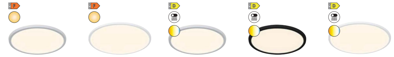
Oja 29 Sensor 2110456101 White | Plastic LED Module 0W | 1600lm | 2700K H: 3,8 cm | Ø: 29,4 cm Oja 42 Sensor 2110476101 White | Plastic LED Module 20W | 2100lm | 2700K H: 3,8 cm | Ø: 42,4 cm Oja 29 2210606101 White | Plastic | LED Module 15W 1700lm | 3000/4000K H: 2,3 cm | Ø: 29,4 cm Oja 29 2210606103 Black | Plastic | LED Module 15W 1700lm | 3000/4000K H: 2,3 cm | Ø: 29,4 cm Oja 42 2210626101 White | Plastic | LED Module 19W 2200lm | 3000/4000K H: 2,3 cm | Ø: 42,4 cm
