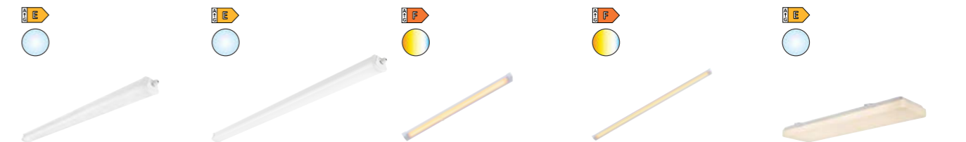
Oakland 120 Double 47746101 White | Plastic LED Module 44W | 4400lm | 4000K H: 6,5 cm | W: 8,3 cm | L: 123,2 cm Oakland 150 Double 47766101 White | Plastic LED Module 55W | 6300lm | 4000K H: 6,5 cm | W: 8,3 cm | L: 153,2 cm Preston 30 2510156101 White | Plastic | LED Module 4W 350lm | 3000/4000K H: 30 cm | W: 3,3 cm | Preston 2510176101 White | Plastic | LED Module 8W 720lm | 3000/4000K H: 55 cm | W: 3,3 cm | Trenton 60 47856101 White | Plastic LED Module 23W | 2500lm | 4000K H: 5 cm | W: 16 cm | L: 60 cm
