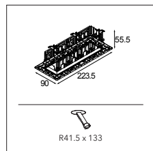
QBINI TRIMLESS FRAME 4X
