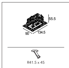
QBINI TRIMLESS FRAME 2X
