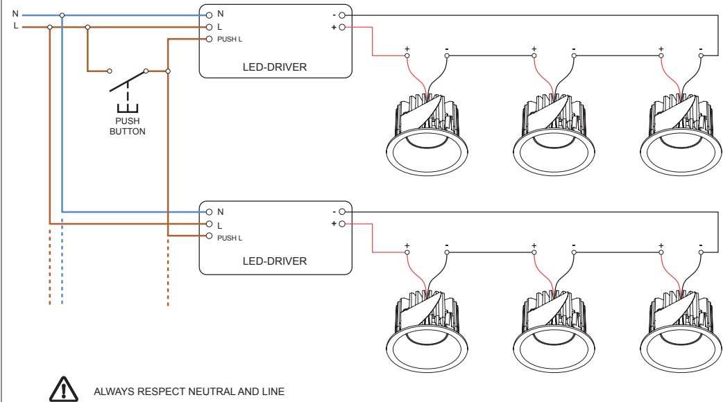
PUSHDIM - SINGLE DIM CHANNEL
