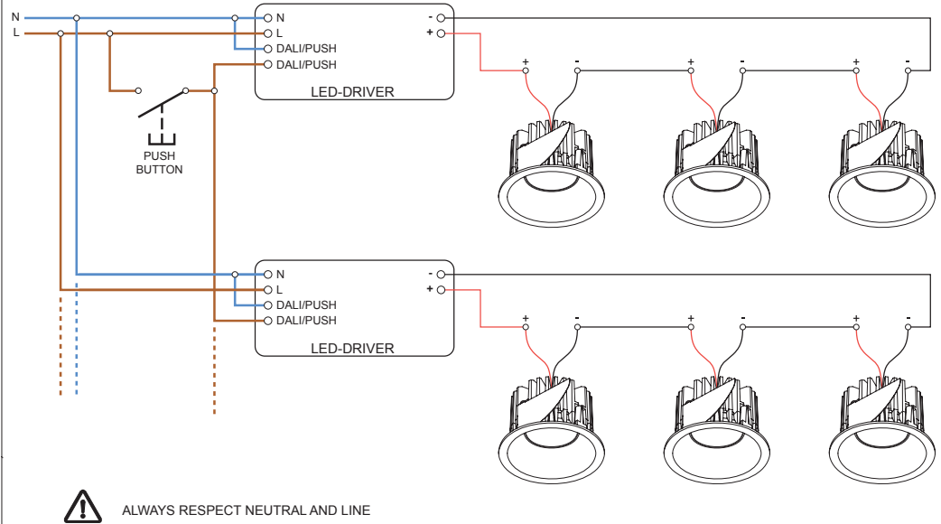
PUSHDIM - DOUBLE DIM CHANNEL
