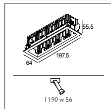
QBINI FRAME 4X
