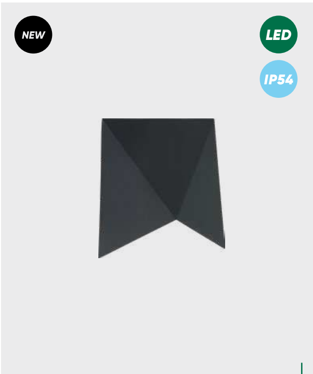
12108 Taifu ↑170mm ↔170mm ↗80mm aluminium-black, glass-clear LED 10W/1000lm, 4000K EAN 8585032240522 LED □ ↻ G A G
