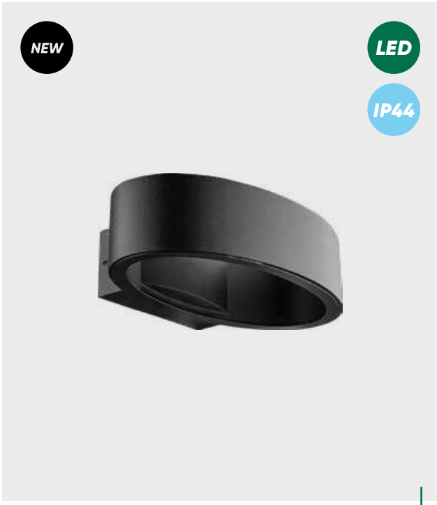
31312 Rebus aluminium-black, glass-clear LED 5W/700lm, 4000K EAN 8585032239533
