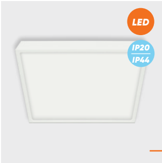
49054 Lenys SQ II. ↓25mm ↔280mm ↗280mm metal-white plastic-white LED 30W/3420lm, 4000K EAN 8585032237416 LED IP20 IP44 LED □ ⚡ F A G
