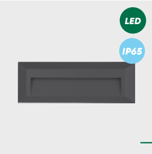
48327 Radix II. ↑80mm ↔230mm ↗27mm plastic-dark grey LED 2.7W/340lm, 4000K EAN 8585032236594 LED □ ↻ E A G
