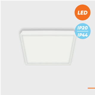
49040 Lenys SQ II. ↓25mm ↔190mm ↗190mm metal-white plastic-white LED 18W/1800lm, 4000K EAN 8585032236358 LED IP20 IP44 LED □ ⚡ F A G
