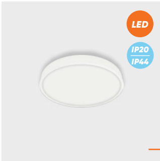
49035 Lenys II. ↓25mm Ø140mm metal-white plastic-white LED 12W/1200lm, 4000K EAN 8585032236303 LED IP20 IP44 LED □ ⚡ F A G
