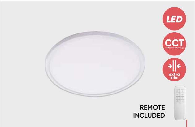
17300 Kraton I. LED CCT extra slim REMOTE INCLUDED metal, aluminium, plastic-matt white LED 18W/1490lm, 2700-6500K EAN 8585032235740 LED G A
