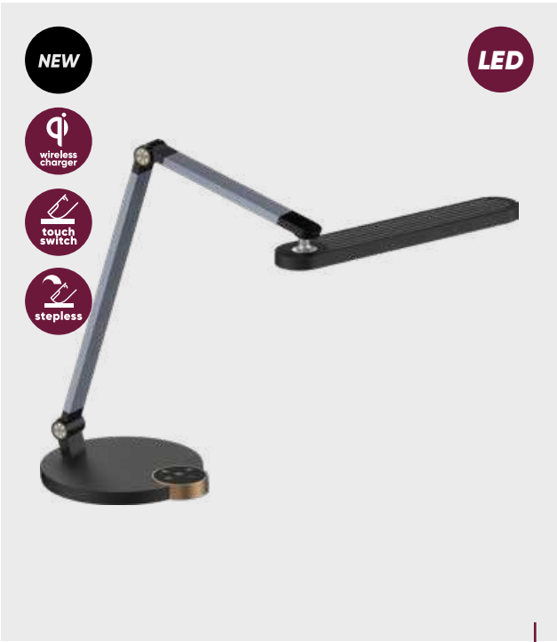
31217 Vivid metal-dark grey brushed ABS-black LED 10W/400-780lm, 3000-6500K EAN 8585032239045 LED, touch switch, stepless, wireless charger F A G
