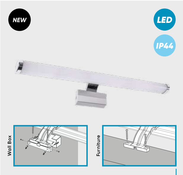
70225 Solana plasticl-chrome acrylic-white LED 12W/1480lm, 4000K EAN 8585032238819
