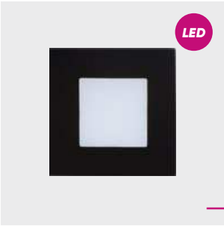
48335 Step light plastic-black LED 1W/60lm, 4000K EAN 8585032237652 86mm 86mm 35mm
