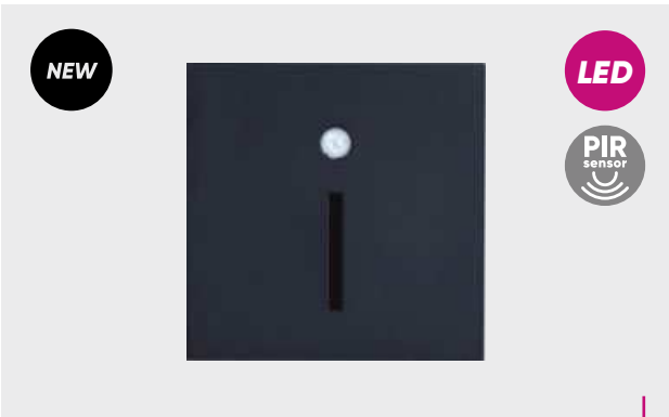
70430 Step light Line S plastic-black LED 1W/20lm, 4000K EAN 8585032238307 LED PIR sensor
