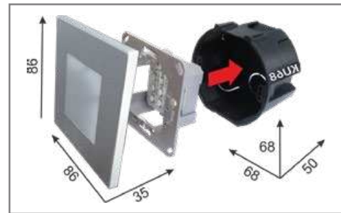
48307 Step light plastic-light wood LED 1W/60lm, 4000K EAN 8585032221521 86mm 86mm 35mm
