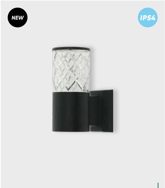
12100 Even 200mm 90mm 150mm aluminium-black, polycarbonate-clear 1xE27/40W EAN 8585032240447 E27 □
