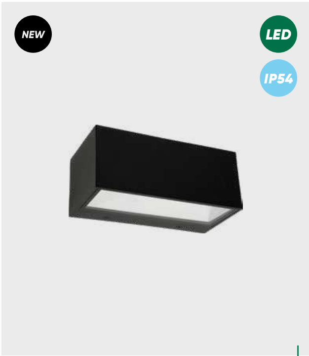
31313 Tanuk aluminium-black, PC-white LED 9W/820lm, 4000K EAN 8585032239540
