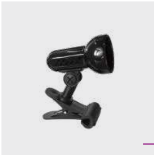
20020 Metro II. ↕120mm ↔100mm metal/plastic-black 1xE14/R50/40W with switch EAN 8590828730040
