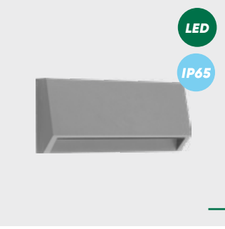
48318 Radix I. ↑70mm ↔160mm ↗33mm plastic-grey LED 3.8W/360lm, 4000K EAN 8585032223563 LED □ ↻ E A G
