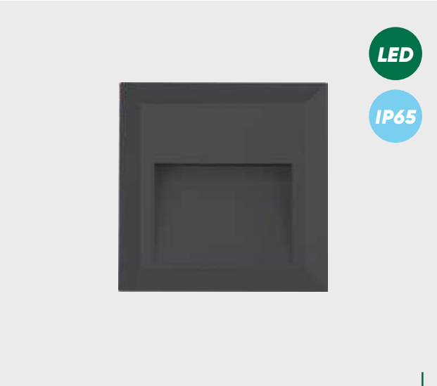
48328 Radix II. ↑125mm ↔125mm ↗27mm plastic-dark grey LED 1.6W/190lm, 4000K EAN 8585032236600 LED □ ↻ E A G
