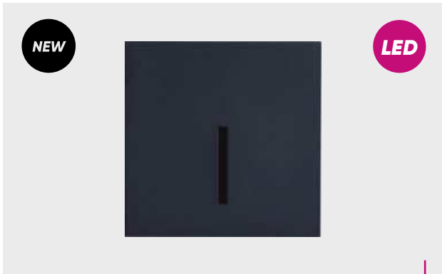
70431 Step light Line plastic-black LED 1W/20lm, 4000K EAN 8585032238314 LED PIR sensor
