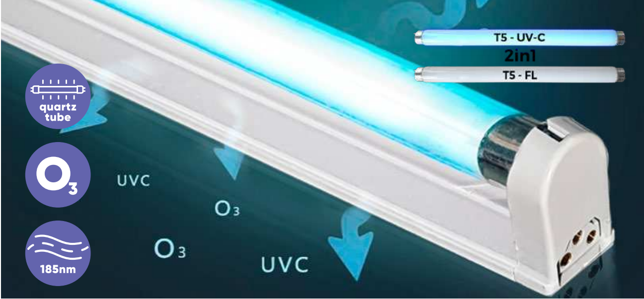
UV 70421 Germicidal tube ↓15mm ↔1163mm ↑15mm T5 UV-C/28W EAN 8585032236563 T5 O 3
