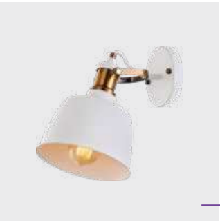
46306 Famosa II. ↓240mm ↔180mm ↗230mm metal-matt white, antique brass 1xE27/40W EAN 8585032234309
