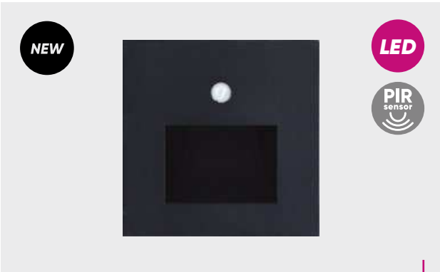
70418 Step light Sunny S plastic-black LED 1W/60lm, 4000K EAN 8585032238185 ø87mm ↔ 87mm 752mm
