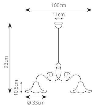
2261.B E27 LED 2 X MAX 10W Lampadina non inclusa / Bulb not included
