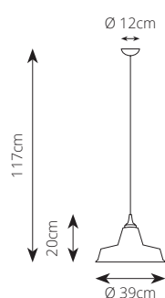
2257.O E27 LED MAX 10W Finitura anticata / Antique finish Lampadina non inclusa / Bulb not included
