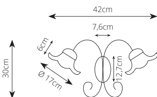
2261.AP2 E27 LED 2 X MAX 10W Lampadina non inclusa / Bulb not included
