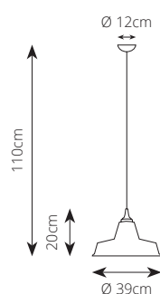
2257.C E27 LED MAX 10W Finitura anticata / Antique finish Lampadina non inclusa / Bulb not included
