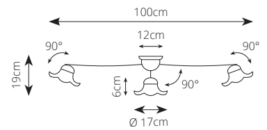
2261.P E27 LED 3 X MAX 10W Lampadina non inclusa / Bulb not included
