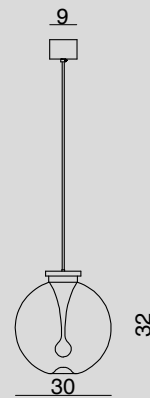
XXL1593.1L SOSPENSIONE A ROSONE / HANGING LAMP WITH CANOPY Glass 1 x Ø 30 cm - Cable 200 cm 1 x LED 12,8 W DIMM
